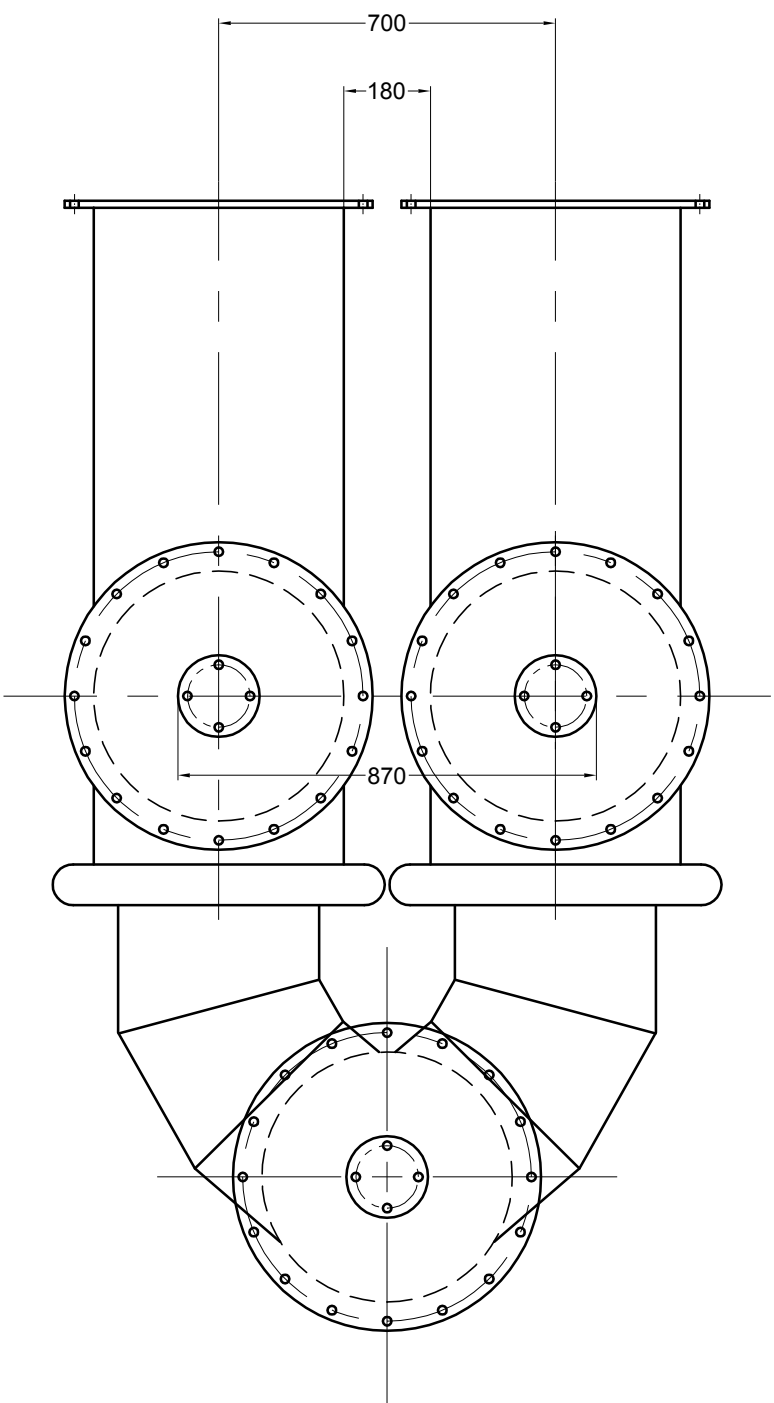
TOP VIEW
