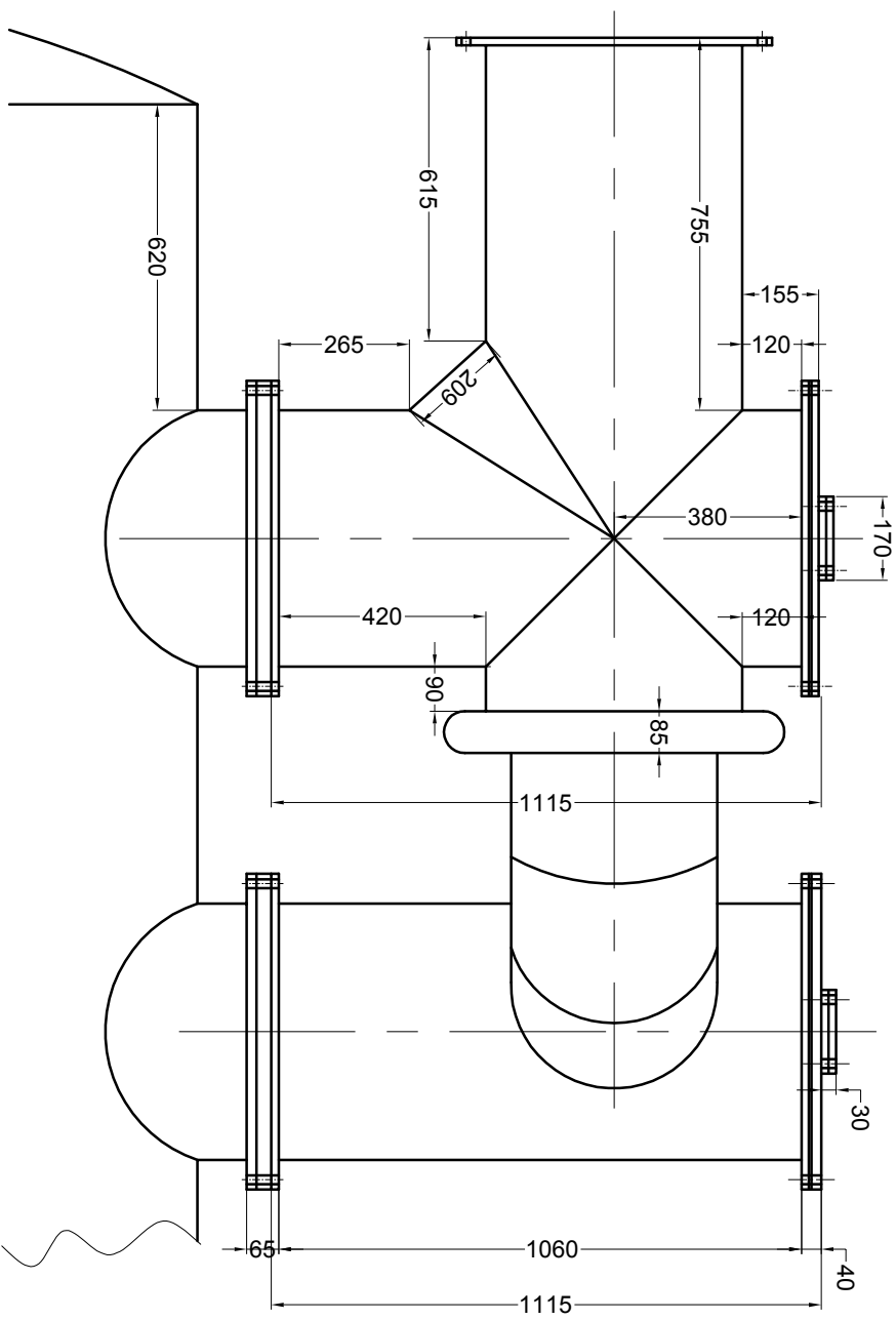
FRONT VIEW
