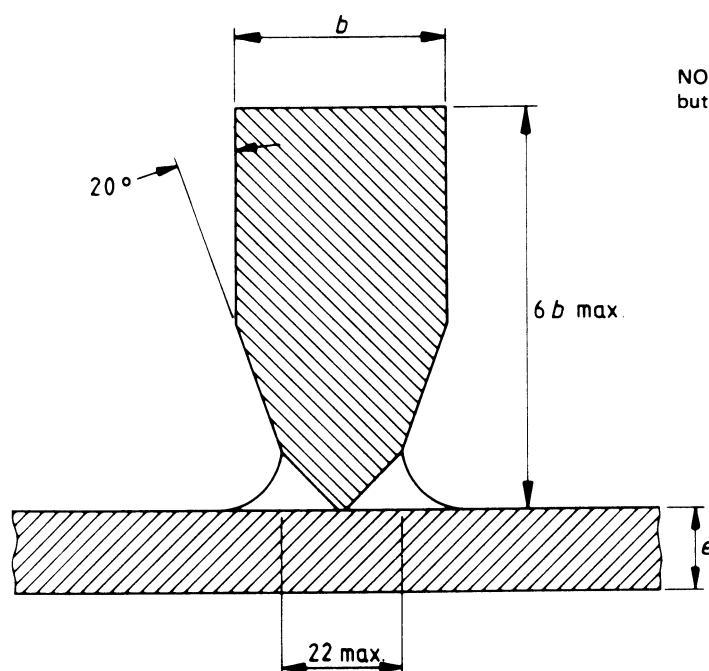
(b) Over 22 mm thick
