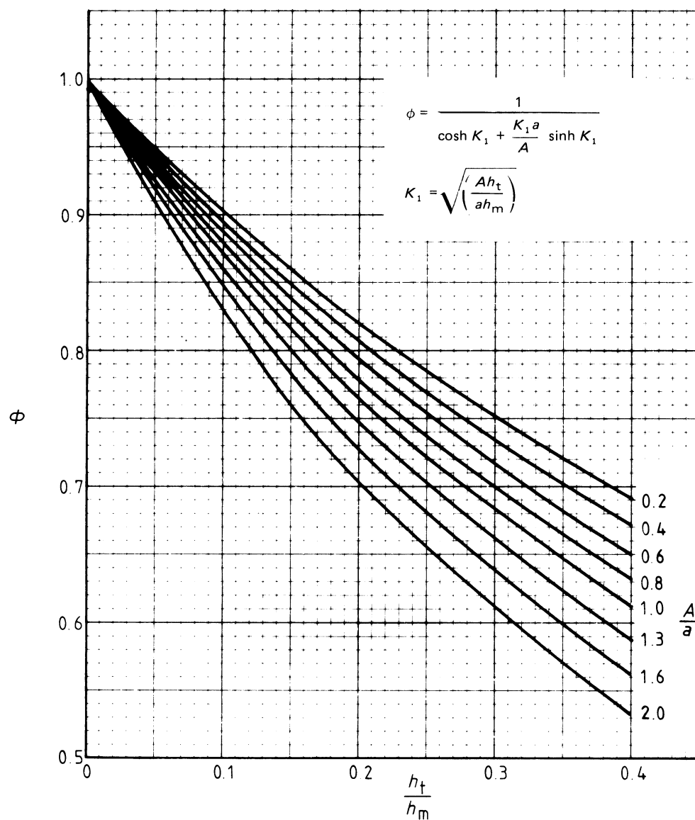
Figure C(11) — Factor \phi
