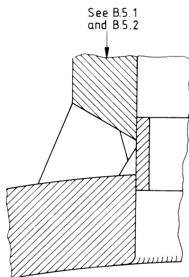
(b) Double root run technique
