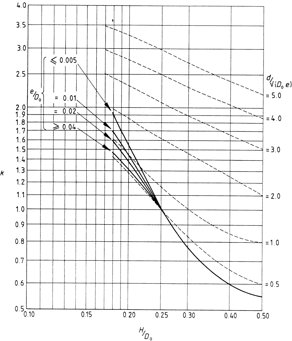
Figure 3.3(2) — Shape factor
