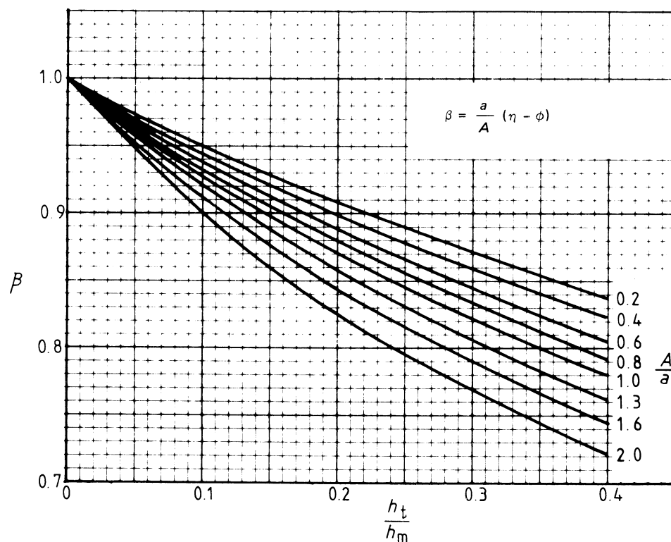
Figure C(12) — Factor \beta
