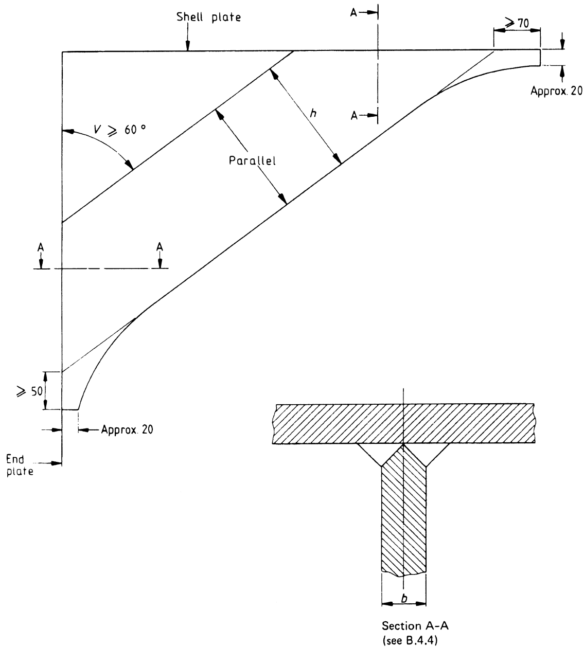
Figure 3.8.8.3(1) — Attachment of welded gusset stays
