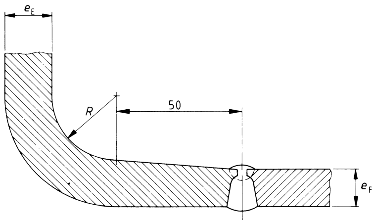
Figure B(5) — Attachment of furnaces to end plates or reversal chamber tubeplates
