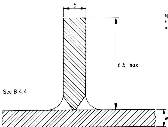
(a) Up to 22 mm thick
