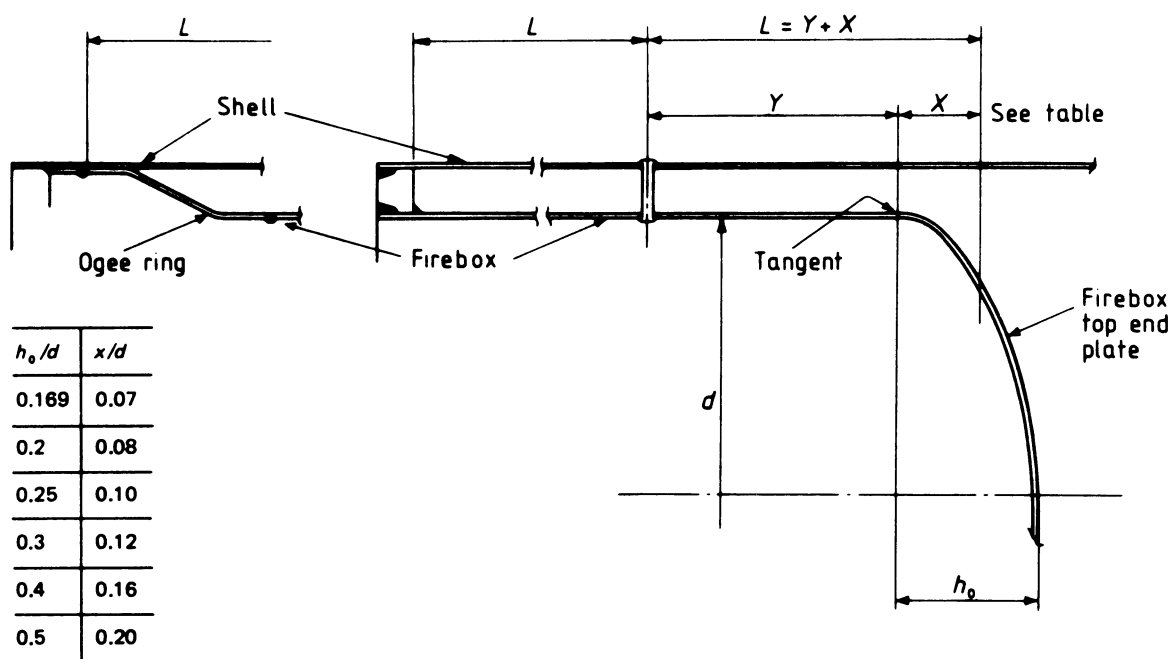
Figure 3.1(5) — Vertical boiler (concluded)
