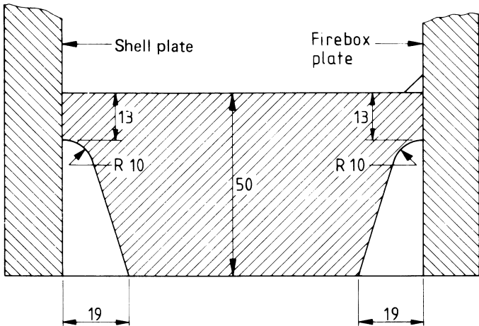
Figure B(9) — Foundation ring
