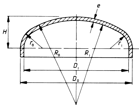
(a) Torispherical end
