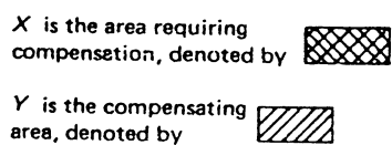
Figure 3.6.1(2) — Compensation for elliptical manholes and inspection openings in flat end plates
