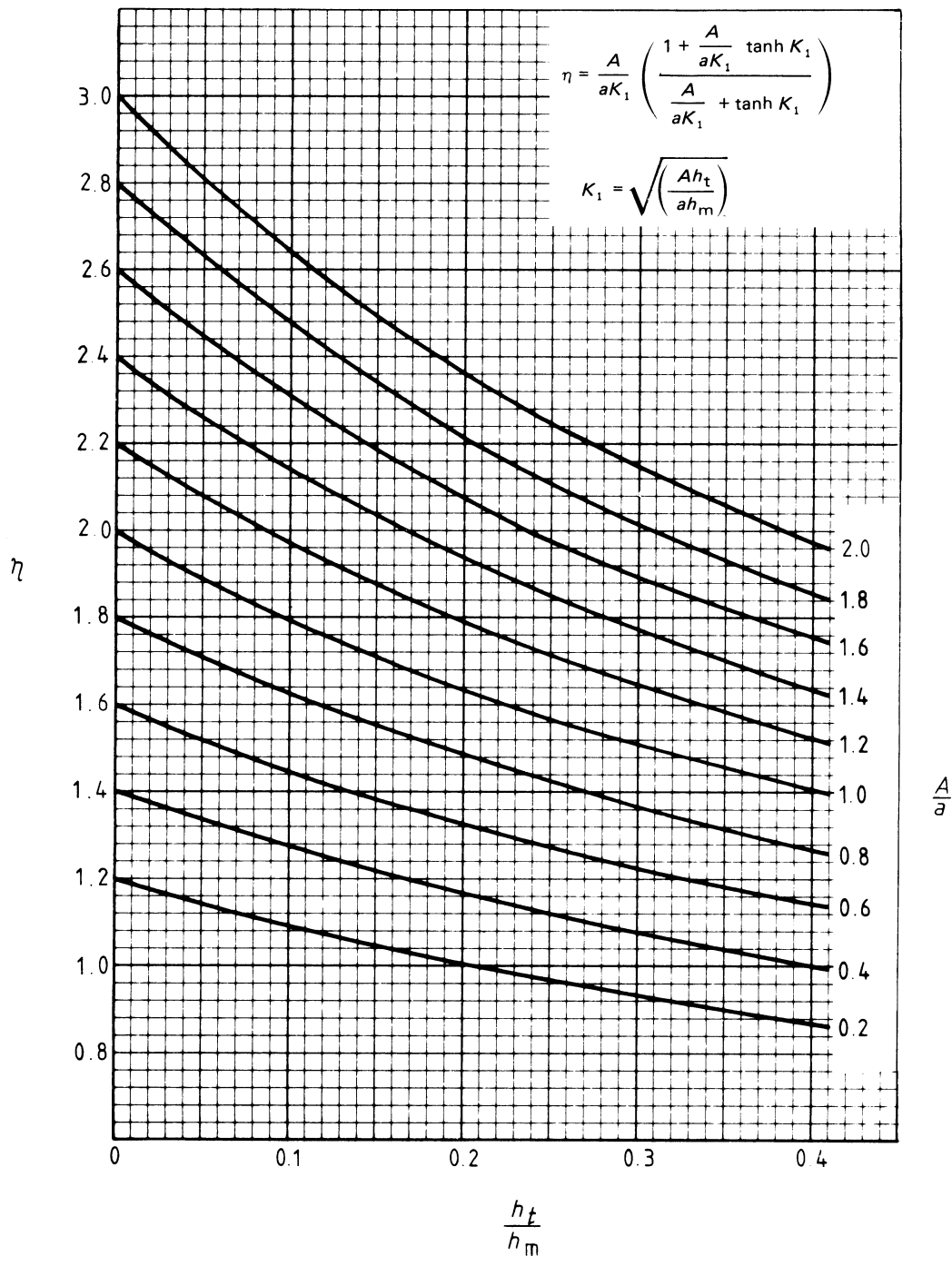
Figure C(10) — Factor \eta
