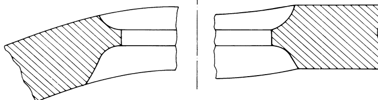
Figure B(18) — Weld details for set-in branches
