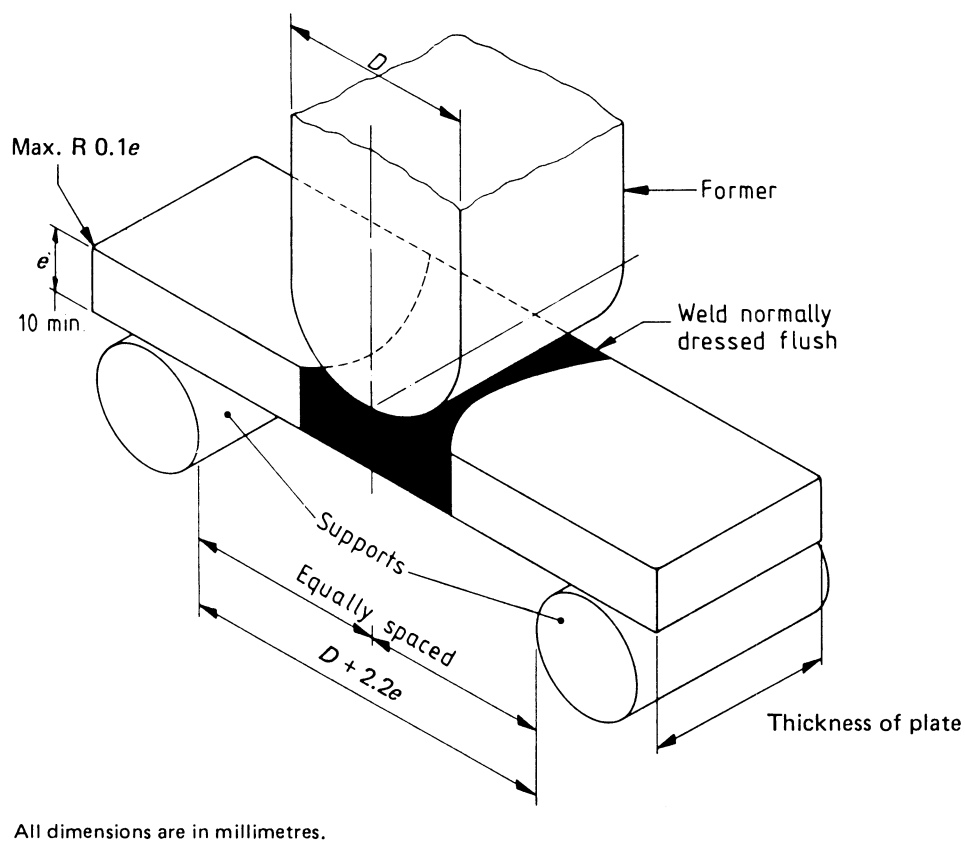
Figure 5.4.7.5 — Side bend test specimen
