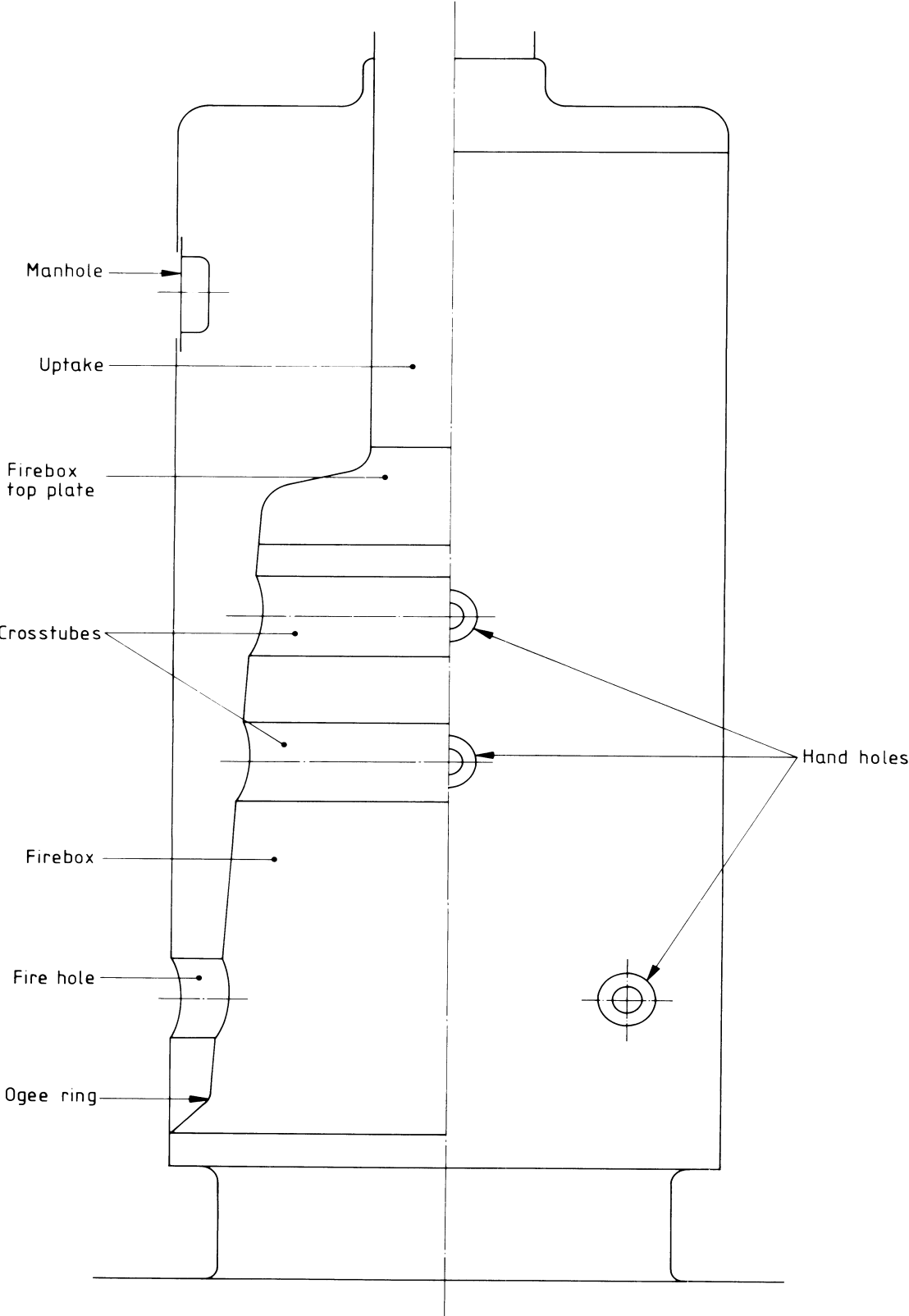
Figure 3.1(5) — Vertical boiler
